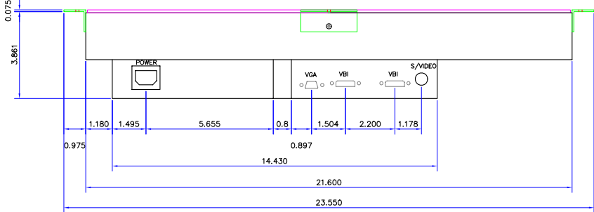
BOTTOM VIEW
