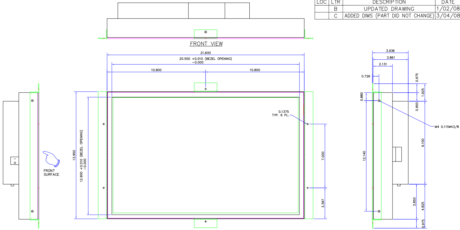
FRONT VIEW
